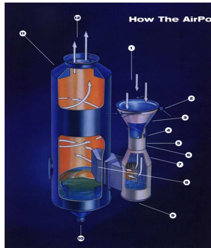
VENTURI SCRUBBERS
