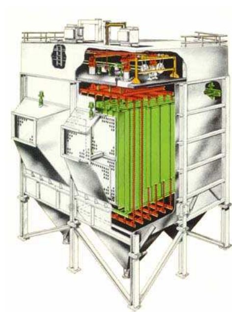
ELECTROSTATIC PRECIPITATORS
