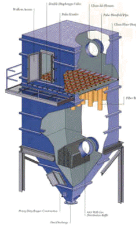
BAG FILTERS
